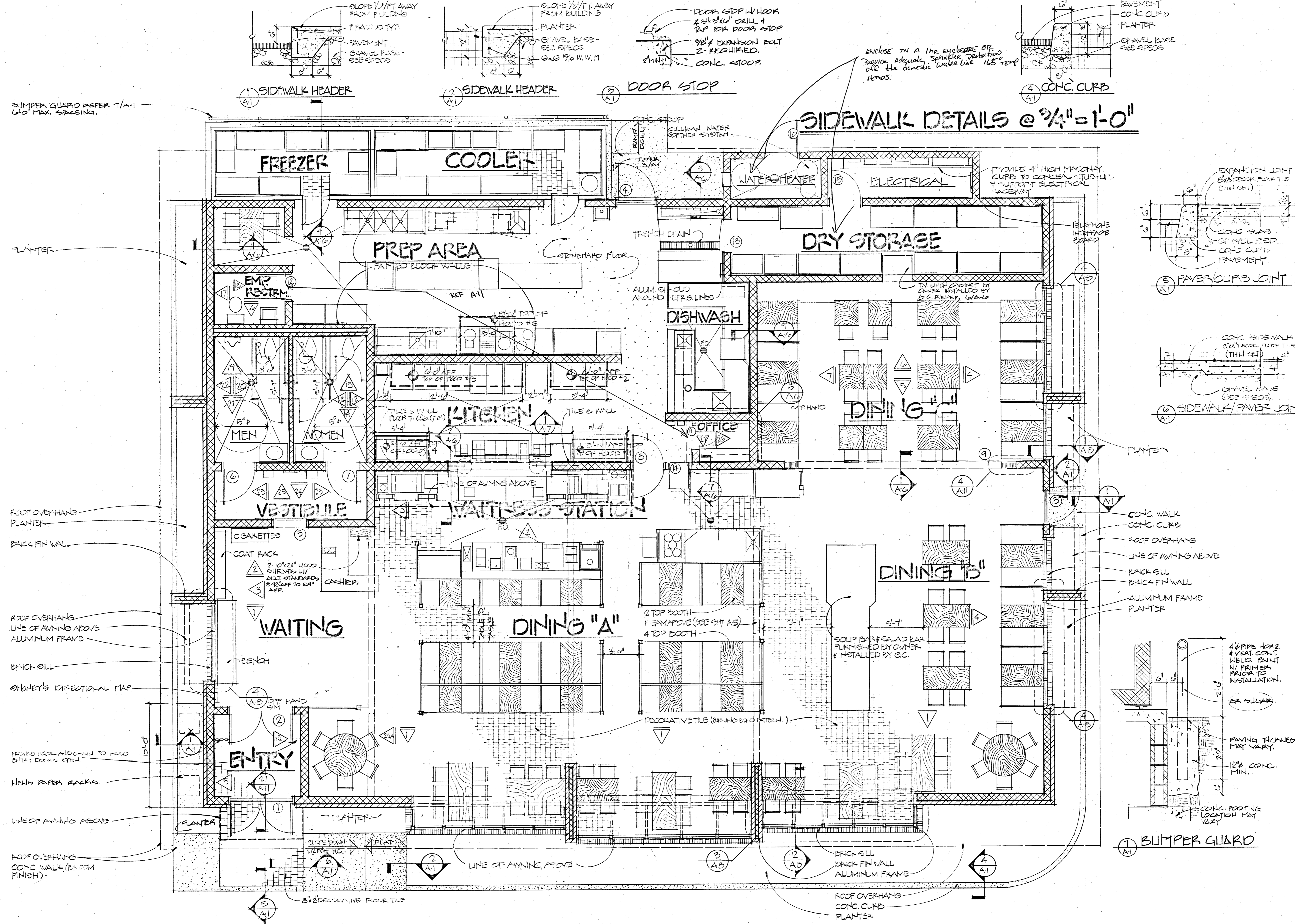
DEPICTIVE FLOOR PLAN @ 1/4" = 1'-0"
